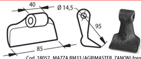
Cod. 18057 MAZZA RM33 (AGRIMASTER, ZANON) foro mm 14,5 Cod. 18060 MAZZA RM33 (SICMA, TIERRE) foro mm 16,5
