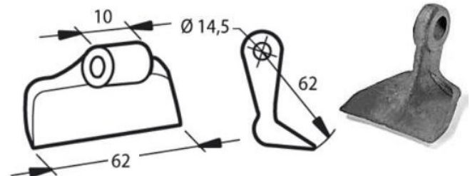
Cod. 18077 MAZZA EU86/14 (ORSI-MAROLIN) foro mm 14,5
