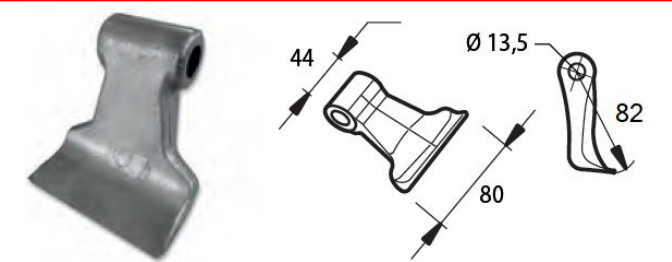
Cod. 18052 MAZZA RM35 (GEO) foro mm 13,5
