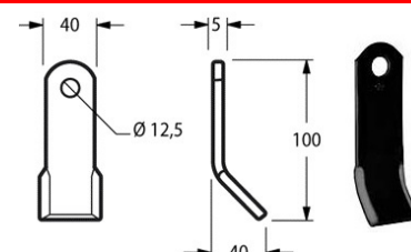
Cod. COLTELLO DECESP. PALLADINO 40x5 {PAL06} 17638
