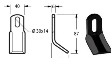
Cod. COLTELLO DECESP. SICMA 40x6 {SIC10} 17665
