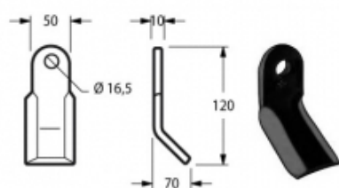
Cod. COLTELLO DECESP. SICMA 50x10 {SIC12} 17666
