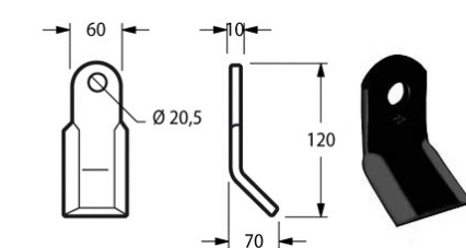
Cod. COLTELLO DECESP. ZAPPATOR 60x10x120 17690 {ZAP03}
