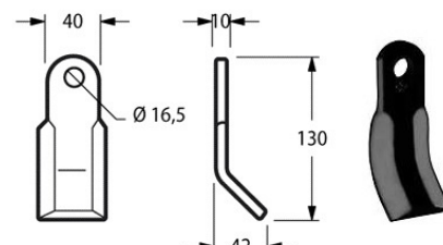
Cod. COLTELLO DECESP. MALETTI-TIERRE 40x10x132 {MAL27}
