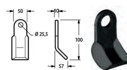
Cod. COLTELLO DECESP. HOWARD 50x10 {HOW48} 17561
