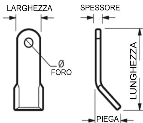
Cod. COLTELLO DECESP. ZAPPATOR 60x10x150 17700 {ZAP01}
