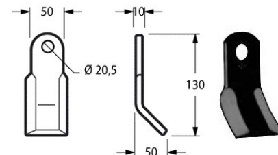
Cod. COLTELLO DECESP. NOBILI BNA 50x10 17610 {NOB12}
