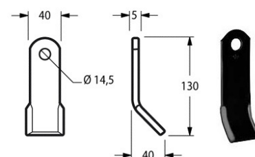
Cod. COLTELLO DECESP. MALETTI FM 40x5 17580 {MAL15}
