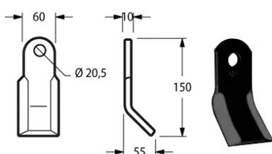
Cod. COLTELLO DECESP. ZAPPATOR 60x10x150 17700 {ZAP01}
