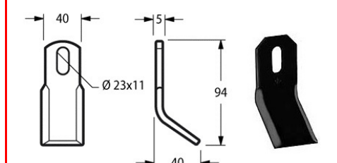
Cod. COLTELLO DECESP. HERMES 40x5 {HER01} 17562
