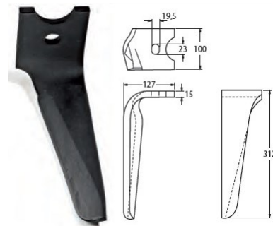
Cod. (Dx/Sx) 06203 - ALPEGO ATTACCO RAPIDO 100x15x312 Ø FORO 23x19,5 [ALP20]
