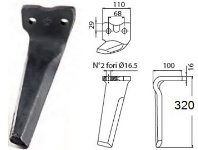
Cod. (Dx/Sx) 06396 - KUHN 110x16x320 INT. 68
