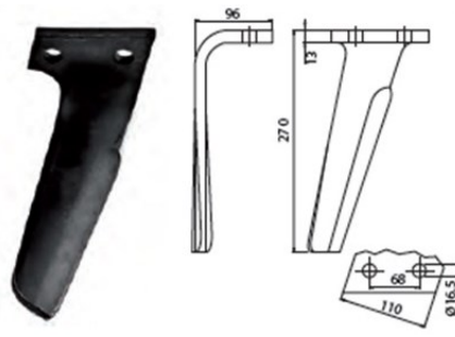
Cod. (Dx/Sx) 06395 - KUHN 525494-5 110x13x270 INT. 68
