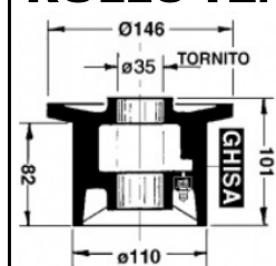
Cod. 03340 RULLO IN GHISA R1
